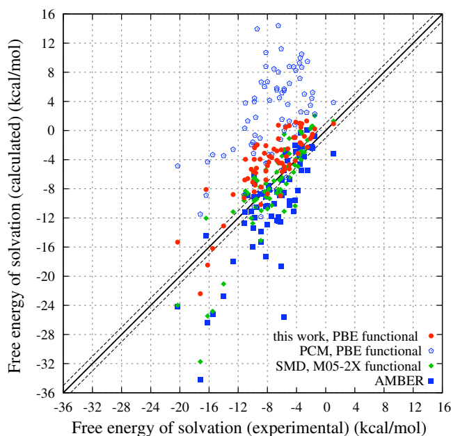
Fig. 4: (Colour on-line) Calculated free energies of solvation plotted against corresponding experimental values for the 71 neutral molecules studied [19,20] — a comparison between models. The solid diagonal line represents perfect agreement with experiment, the dashed black lines denote the estimated uncertainty in the experimental values.
